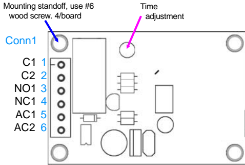
Fig 1: Timer-1 Basic Connections
