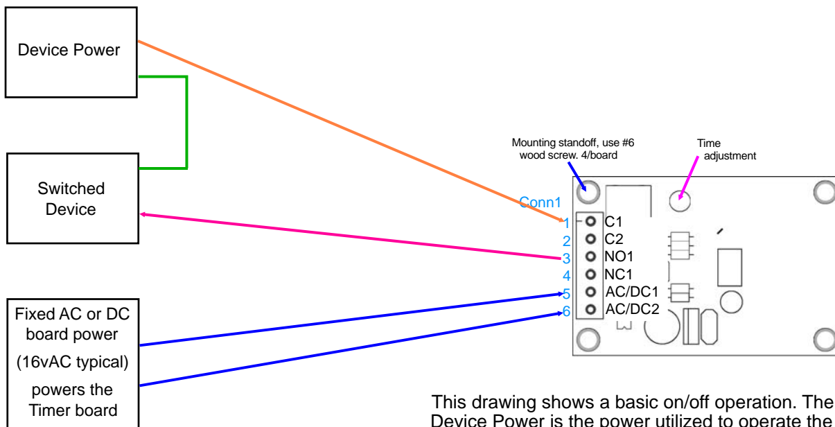
Fig 2: On / Off Operation
