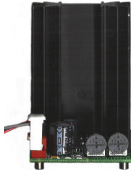
Item 672, 22 Watt amplifier Measures 1 3/4" x 1 3/4" x 3"
