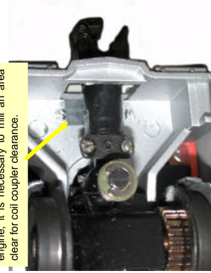
Coil Couplers
