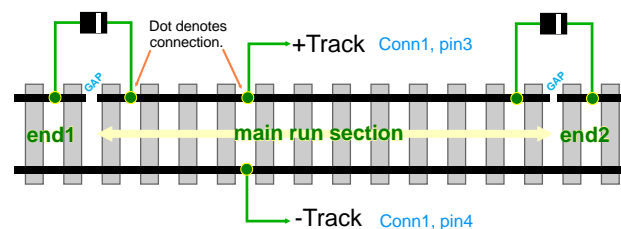
Fig 2: Standard track wiring
